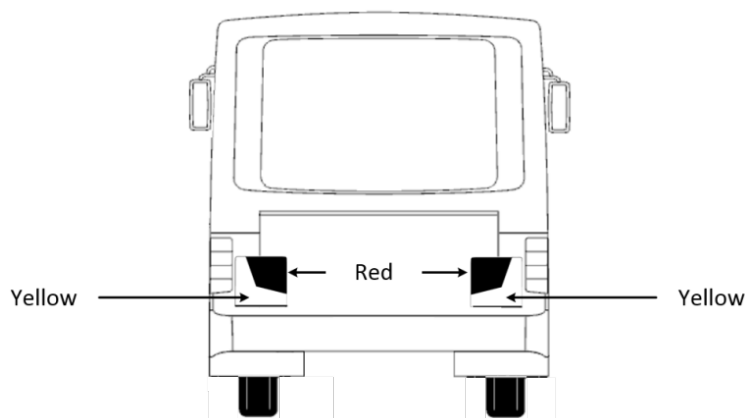
An example of rear marking plates
